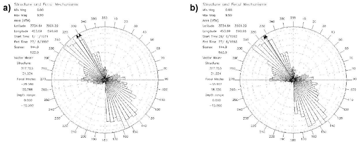
Figure 14. Relation between fault structure and seismic data. In each diagram, the upper quadrant shows the number 1 km long fault segments binned at 5^\circ intervals between -90^\circ and 90^\circ , and the lower portion of the diagram shows the number of earthquake nodal planes binned at 5^\circ intervals between 90^\circ and 270^\circ (where the nodal plane of each focal mechanism most consistent with the regional trend is chosen). Earthquake data are the same as plotted in Figure 1. Arrows represent vector means of both data sets. (a) Preshocks with vector mean of structure of 327.8^\circ , whereas vector mean of preshocks is 330.9^\circ . (b) Aftershocks with vector mean of structure of 327.8^\circ , whereas vector mean of preshocks is 326^\circ .
